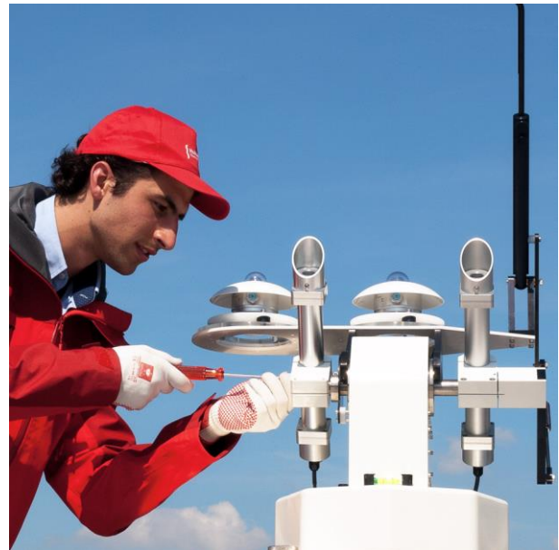
Figure 2 Typical reference measurement station with a solar tracker, pyrheliometers model DR02 and pyranometers model SR20
